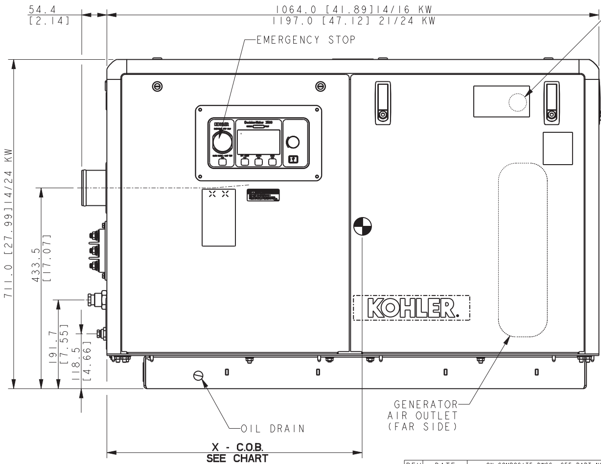
SOUND SHIELD WITH REAR CONNECTION PANEL
