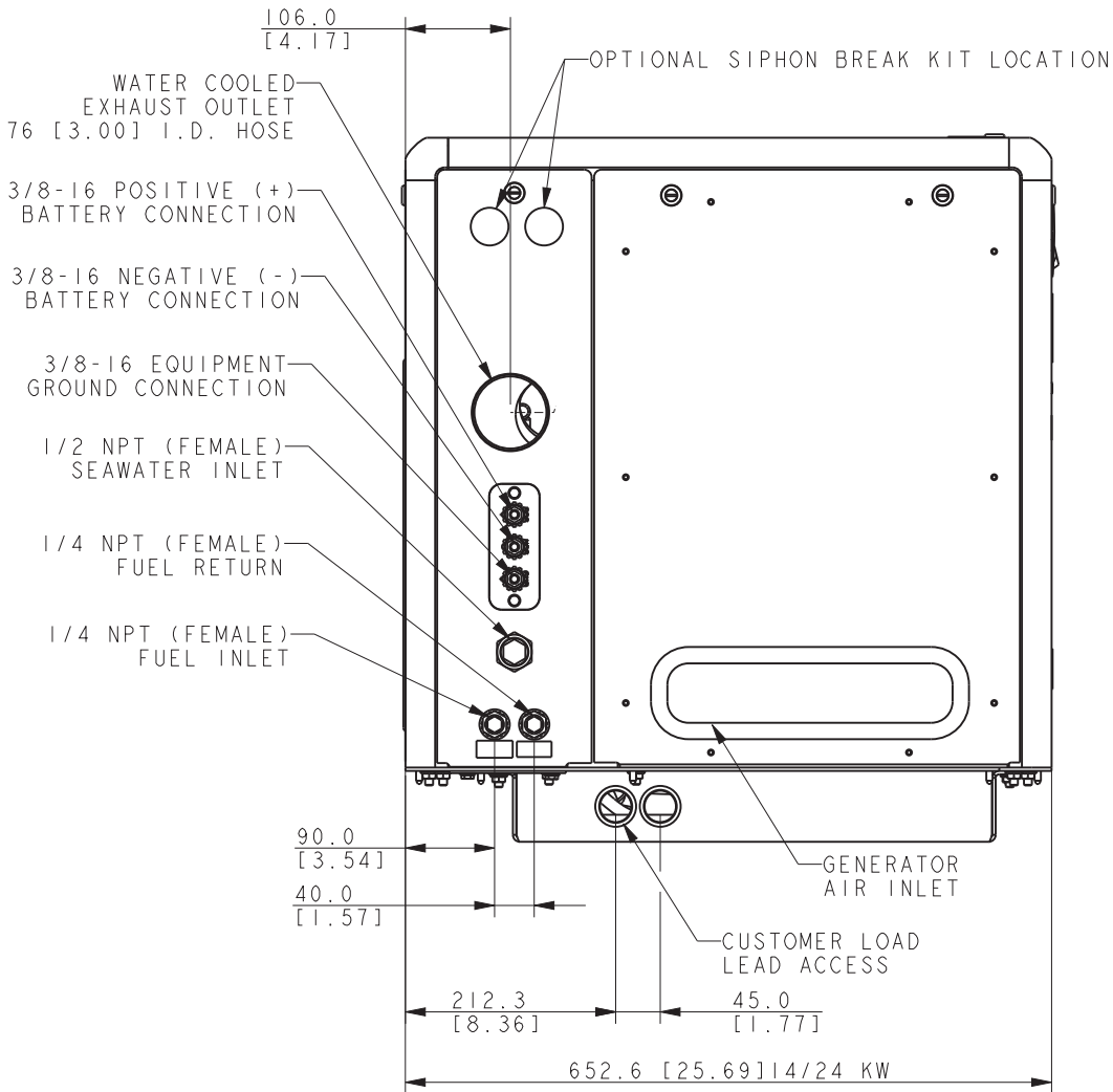
SOUND SHIELD WITH REAR CONNECTION PANEL
